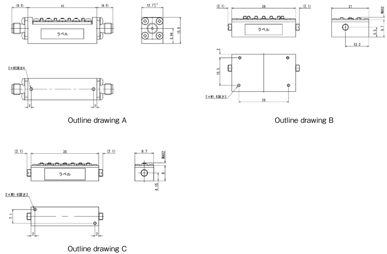
Outline drawing
