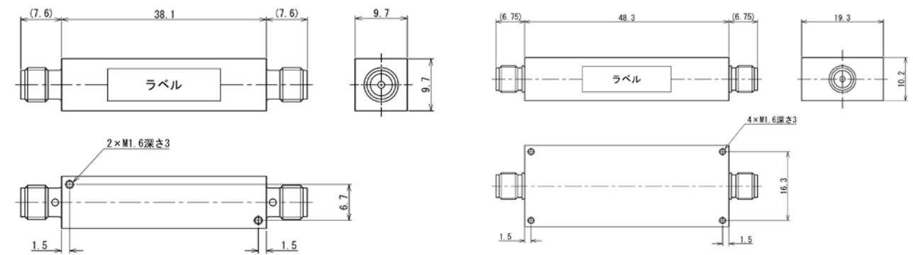
Outline drawing
